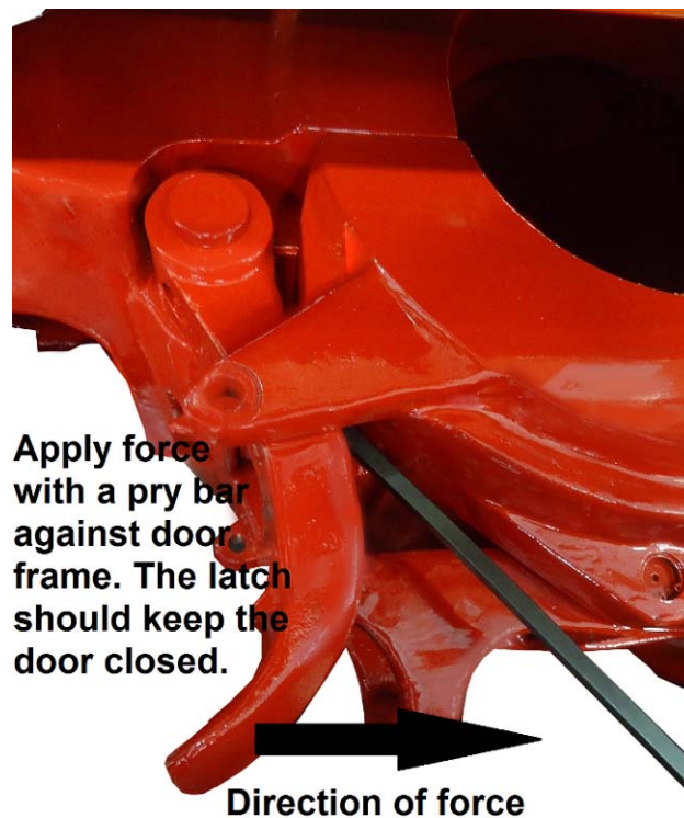
Figure 4: Pry Test Instruction SX
